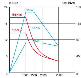
A2-8机械主轴功率扭矩图 A2-8Power-Torque Chart of the Mechanical Spindle
