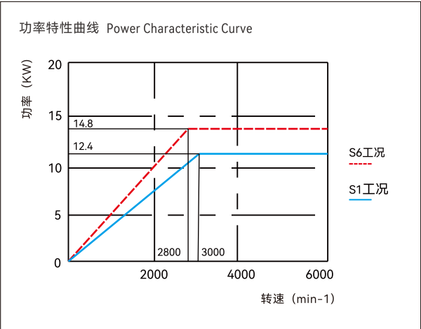
A2-4电主轴功率扭矩图 A2-4 Electric Spindle Power-Torque Chart
