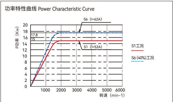
A2-5电主轴功率扭矩图 A2-5 Electric Spindle Power-Torque Chart
